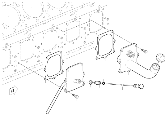
INSPECT PORT COVER FOR OIL DIPSTICK XS527010.00005
